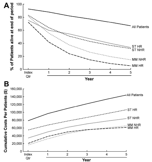
Fig 18. (A) Survival for 3,624 Medicare patients treated in 2003 for isolated aortic valve stenosis. The 5% random sample showed 31% were treated medically, 651 were categorized as high-risk medically treated. The associated variables in the 651 medically treated high-risk patients were central nervous system or psychiatric disease 53%, unstable angina 43%, prior surgery 40%, peripheral vascular disease 28%, chronic pulmonary disease 22%, pulmonary hypertension 20%, and cancer 18%. These variable likely influenced the decision not to operate. The curves show the 5-years survivals. (HR = high risk; MM = medically managed; NHR = not high risk; ST = surgical treatment.) (B) Cost of care over 5 years for those operated on or treated in 2003. Costs are Medicare payments for Parts A, B, and schedule beneficiary cost sharing.
